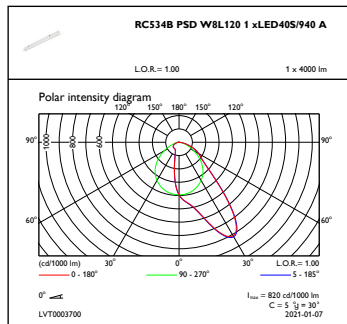
OFPC1_RC534BPSDW8L1201xLED40S940A
