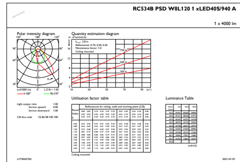
IFGU1_RC534BPSDW8L1201xLED40S940A
