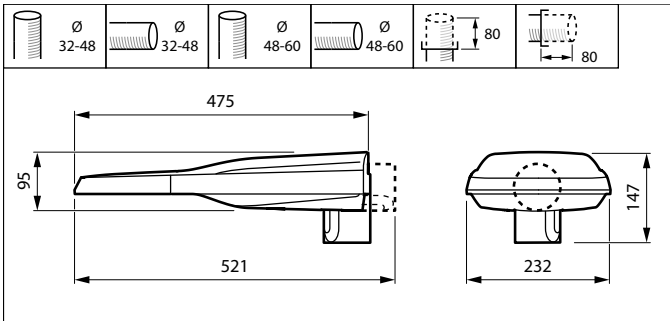
BGP281 LED35-4S/740 I DN10 DDF2 D18 SRG1
