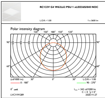
OFPC1_RC133VG4W62L62PSU1xLED36S840NOC
