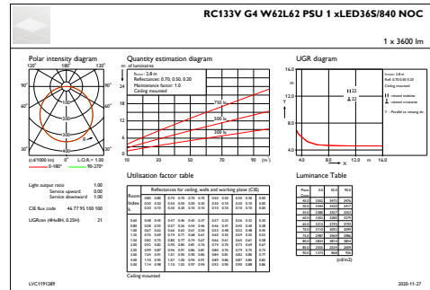
IFGU1_RC133VG4W62L62PSU1xLED36S840NOC
