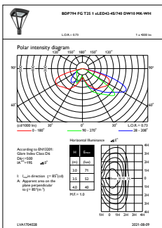
OFPL1_BDP794FGT25xLED42-4S740DW10MK-WH
