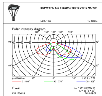
OFPC1_BDP794FGT25xLED42-4S740DW10MK-WH
