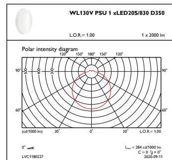
OFPC1_WL130VPSU1xLED20S830D350
