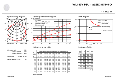
IFGU1_WL140VPSU1xLED34S840O
