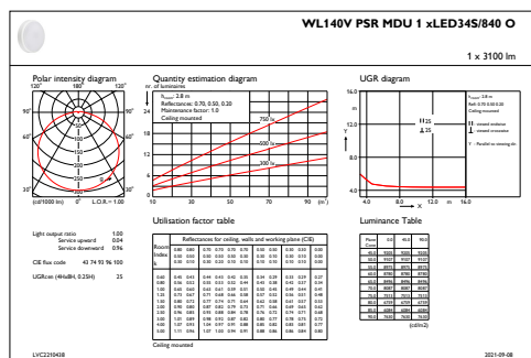
IFGU1_WL140VPSRMDU1xLED34S840O
