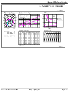
MC LEDtube 25W G13 3700lm 840
