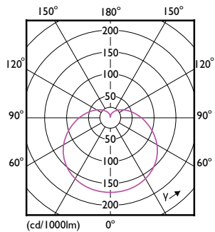
Light Distribution Diagram - LEDbulb ND 13-100W A67 E27 827 2CT
