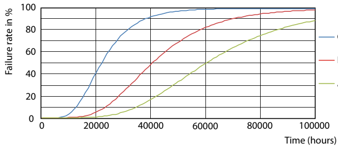
LEDtube_60K_FailureRate
