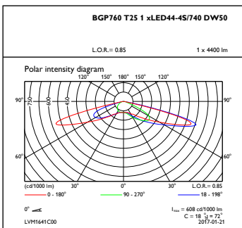
OFPC1_BGP760T251xLED44-4S740DW50
