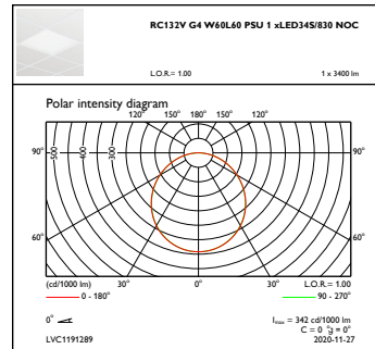
OFPC1_RC132VG4W60L60PSU1xLED34S830NOC
