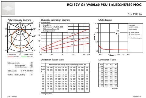
IFGU1_RC132VG4W60L60PSU1xLED34S830NOC
