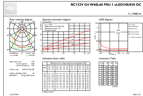
IFGU1_RC132VG4W60L60PSU1xLED345830OC
