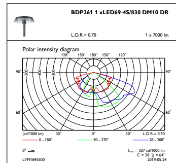
OFPC1_BDP2611xLED69-4S830DM10DR
