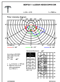
OFPL1_BDP2611xLED69-4S830DM10DR
