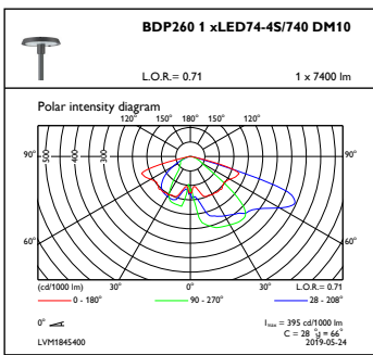
OFPC1_BDP2601xLED74-4S740DM10
