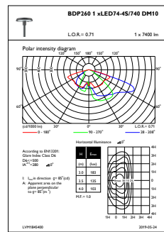
OFPL1_BDP2601xLED74-4S740DM10
