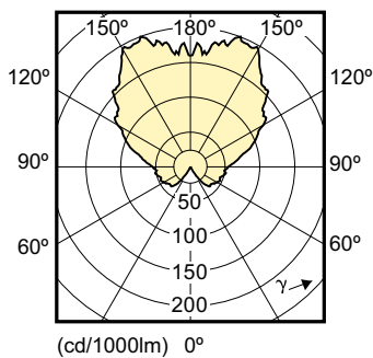
LED DimTone 8-60W 827 806lm
