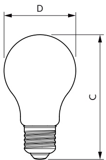
A60 230V 100W 1521lm 2700-2200K E27 D CL
